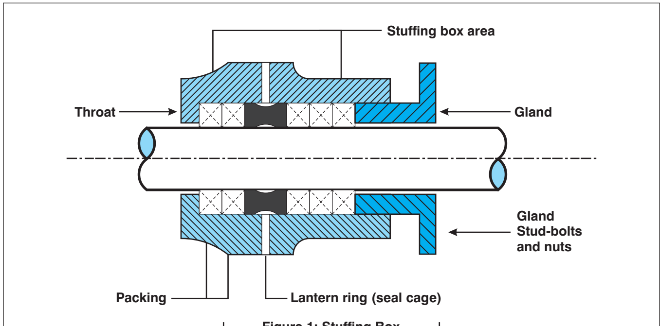
Figure 1: Stuffing Box
